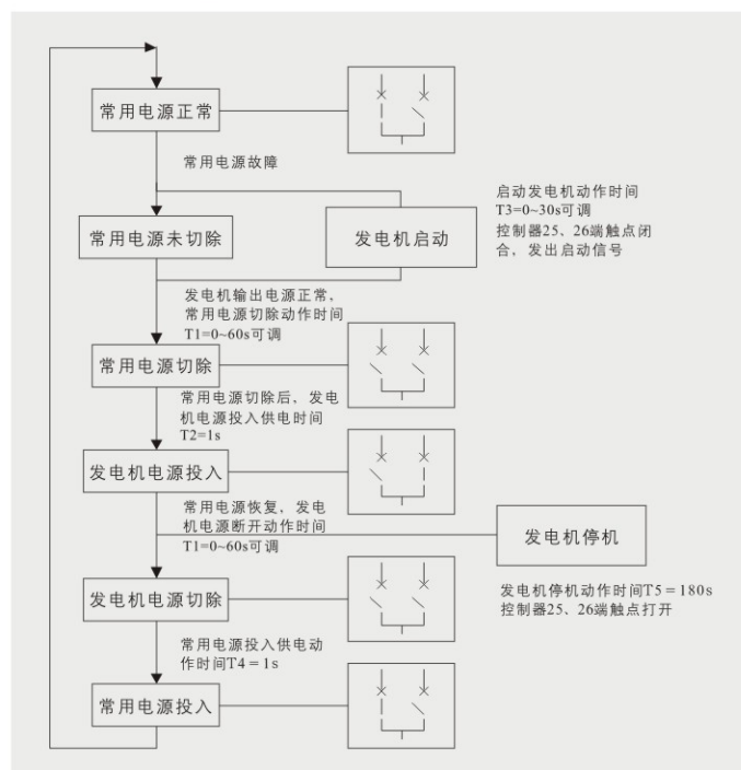
电网-发电机型自投自复功能逻辑图
